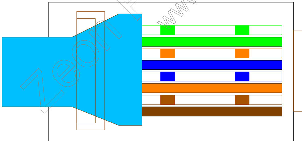
T568A Colors
