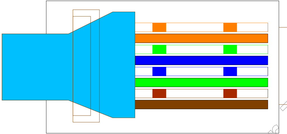
T568B Colors
